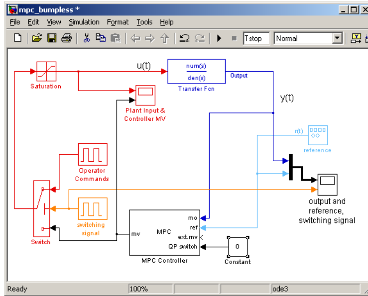
Figure 4-33: External Manipulated Variable Feedback Disconnected
